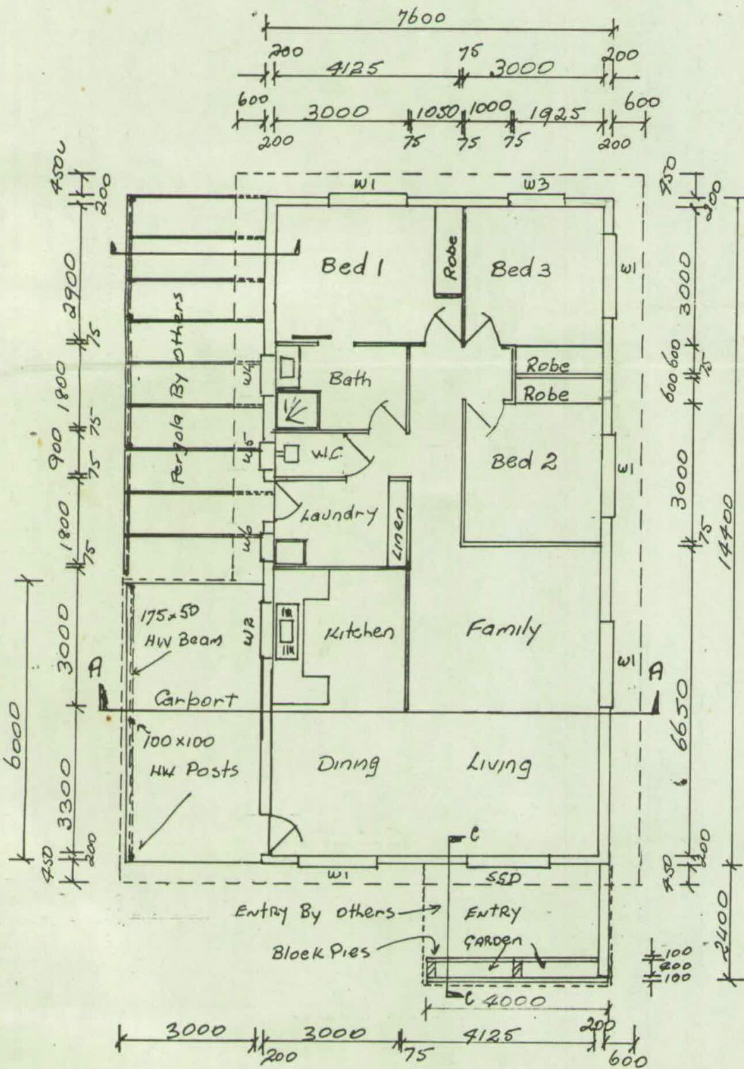
Floor Plan
