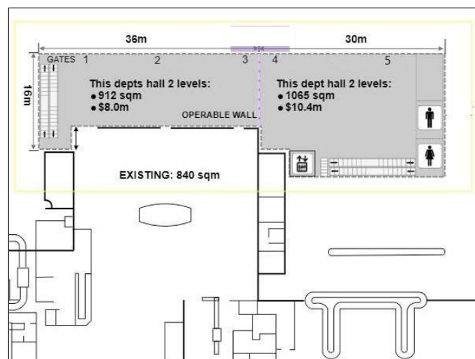
Figure 7: Proposed departures hall expansion concept.
