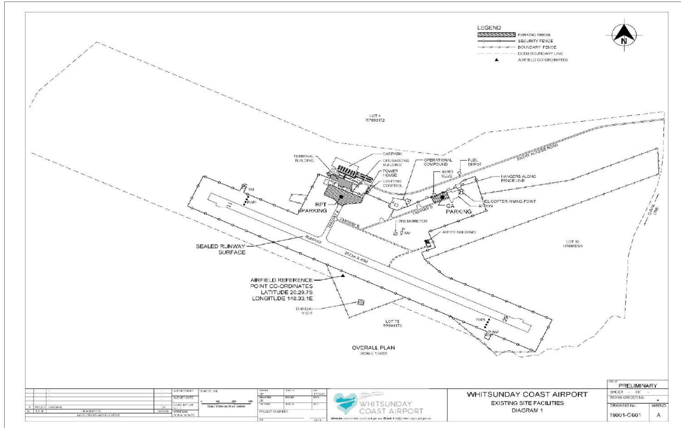
Figure 6: Existing airport site facilities (A3 size)
