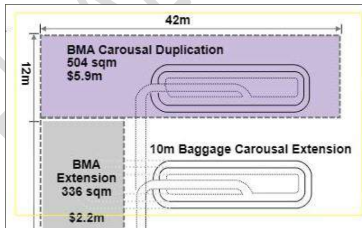
Figure 12: BMA carousel duplication concept.
