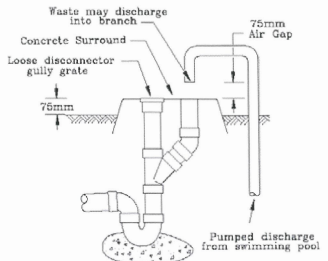
TYPICAL CONNECTION OF PUMPED WASTE DISCHARGE FROM SWIMMING POOLS
