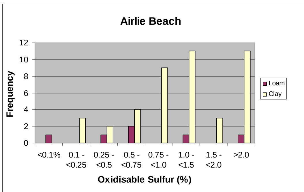
Figure 2. Frequency of PASS samples within oxidisable sulfur ranges for the loam and clay ASS texture groups
